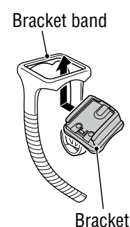
Bracket
